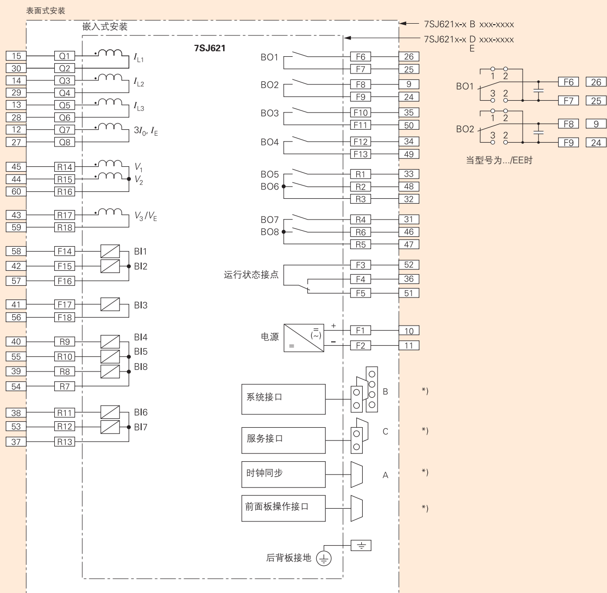
图5/102: 7SJ621接线图
